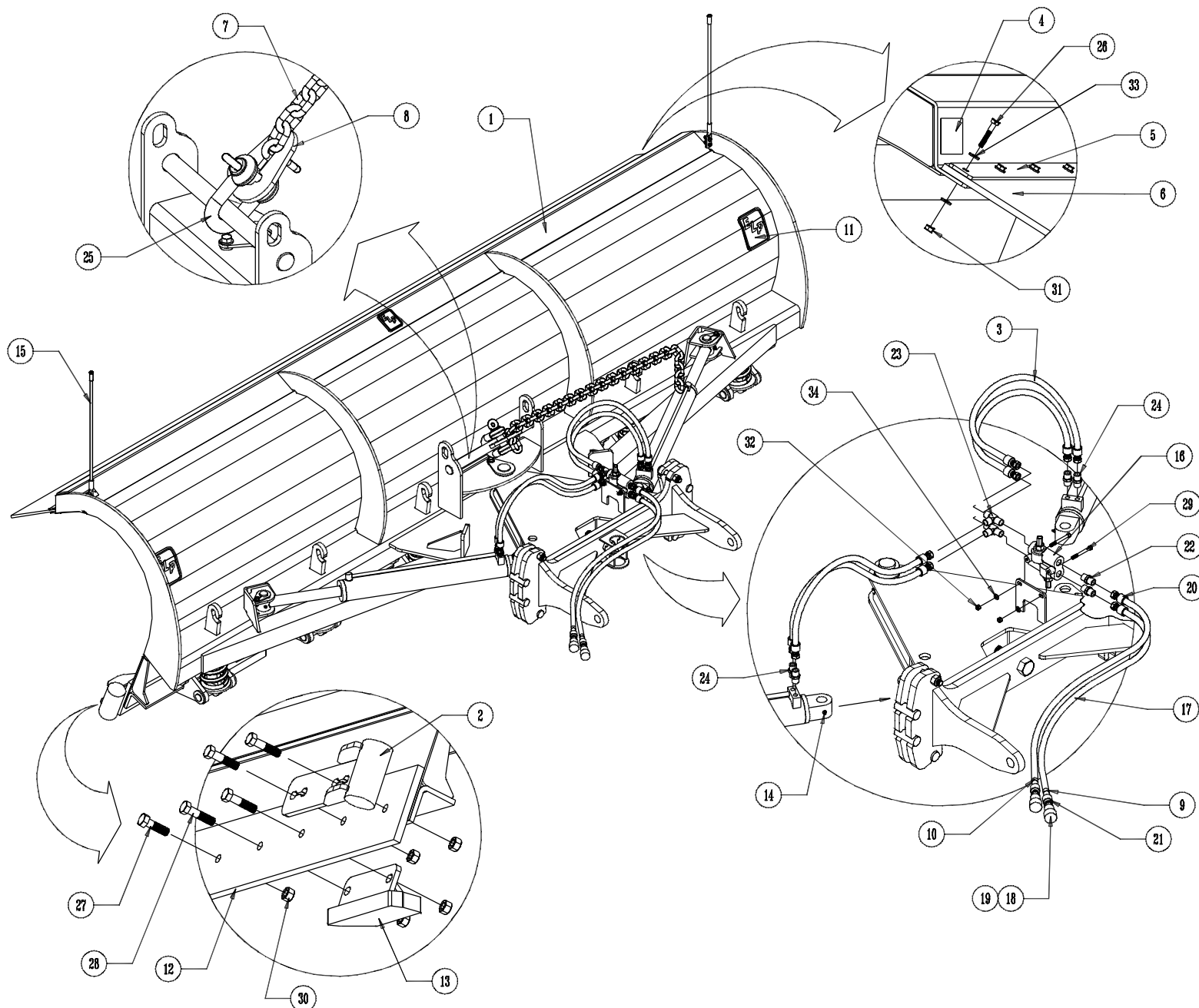
ENSEMBLE FINITION REVERSIBLE 12-36 LANE STANDARD / STANDARD BLADE 12-36 REVERSIBLE ASSEMBLY
