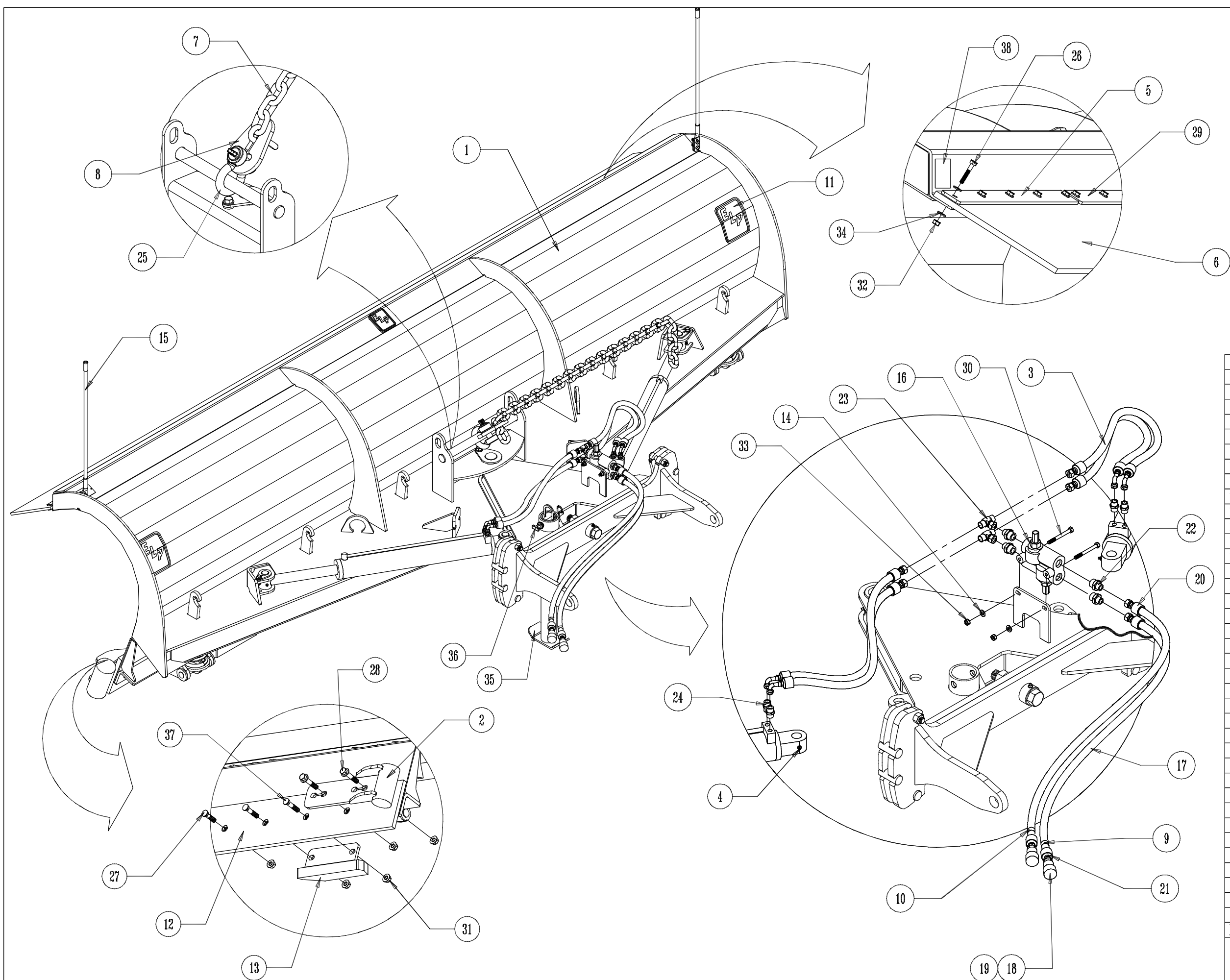
ENSEMBLE FINITION REVERSIBLE LEGER 11-30 T2 / T2 11-30 LIGHT REVERSIBLE FINITION ASSEMBLY
