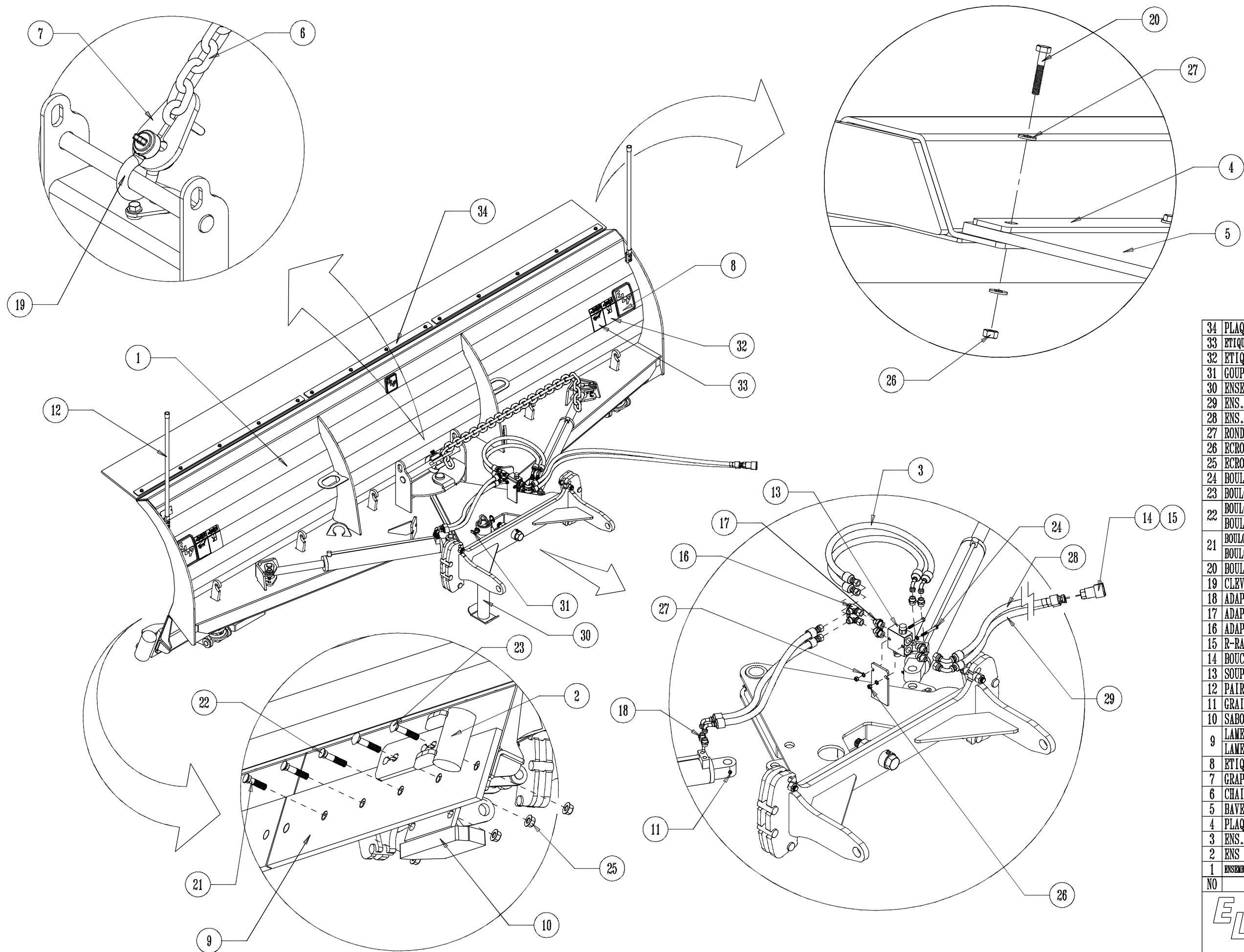
ENSEMBLE FINITION REVERSIBLE LEGER 11-35 T2-1 / T2-1 11-35 LIGHT REVERSIBLE FINAL ASSY
