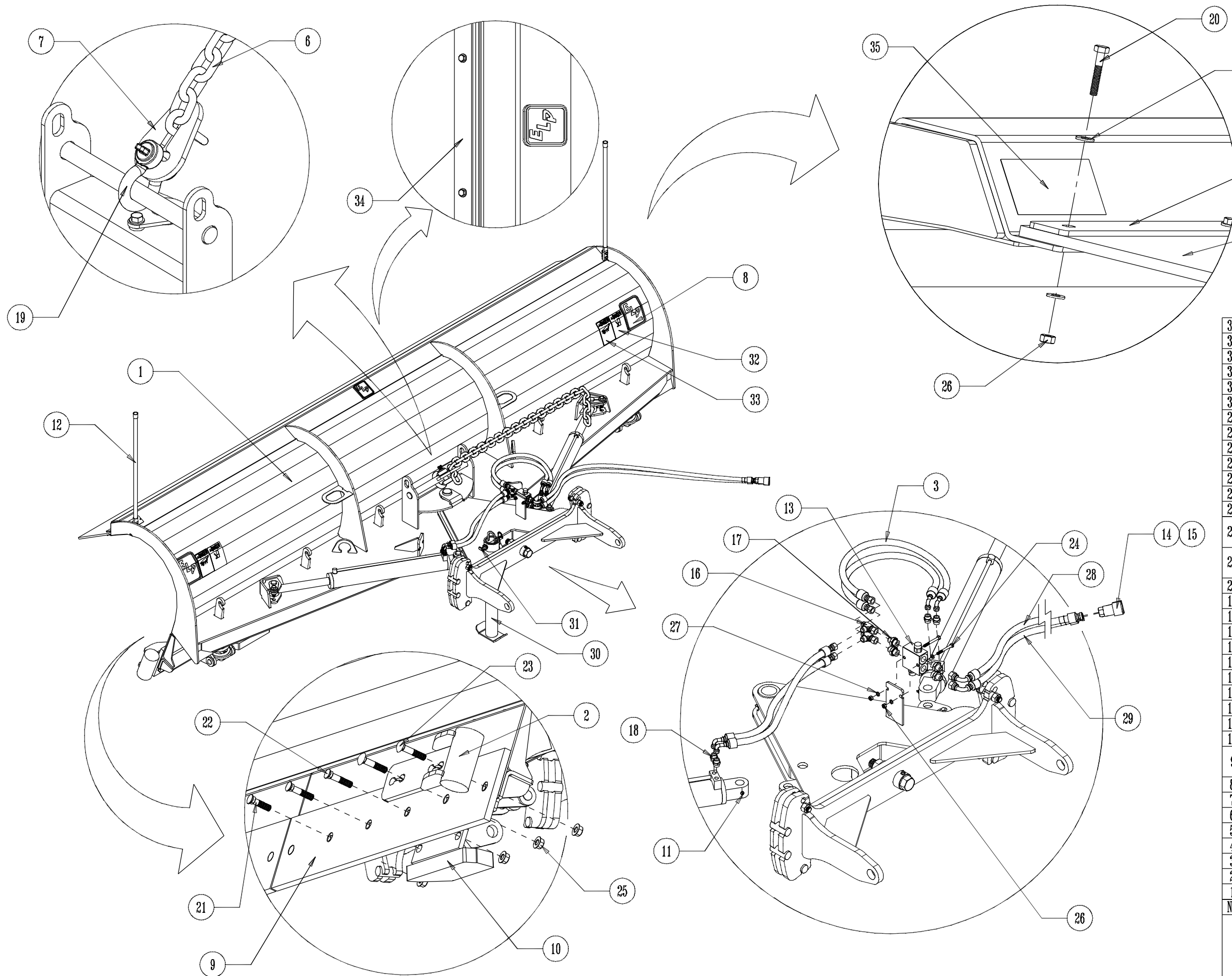
ENSEMBLE REVERSIBLE LEGER 11-30 T2-1 / T2-1 11-30 LIGHT REVERSIBLE ASSY
