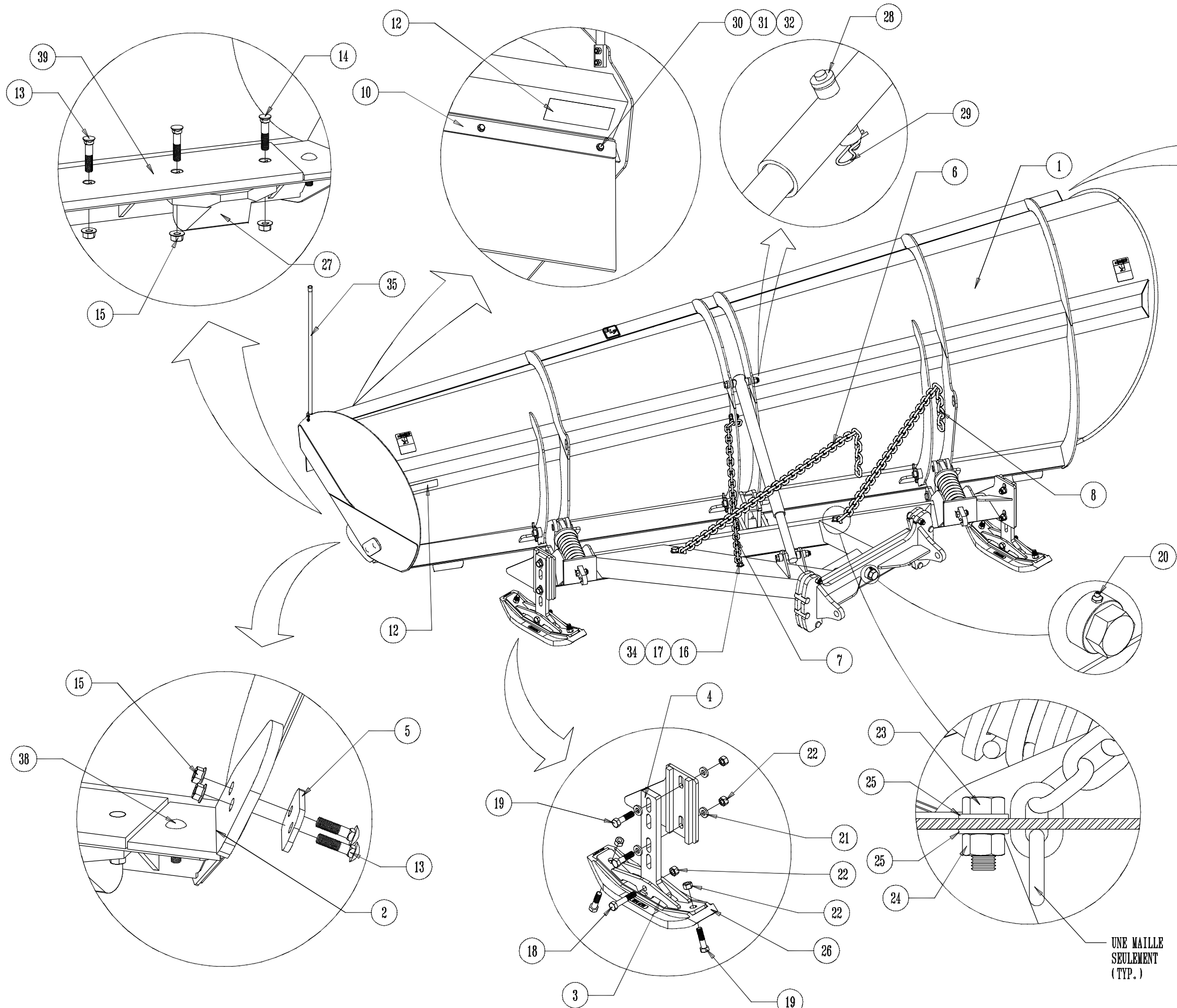
ENSEMBLE FINITION SENS UNIQUE 12-30-55 T2 / 12-30-55 T2 ONE WAY FINITION ASSEMBLY
