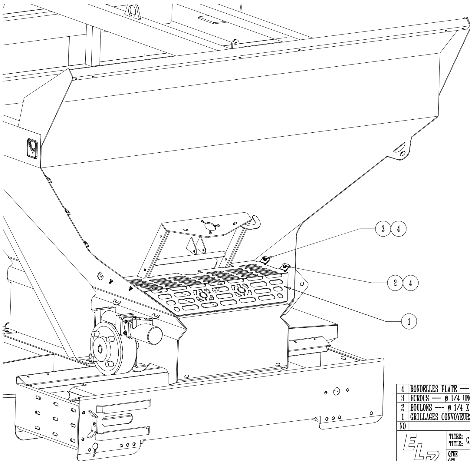
ENSEMBLE GRILLAGE AVANT CONV. SAB. STD. ELP. / ELP STD. SPD. LONG. CONV. FRONT SCREEN ASSEMBLY
